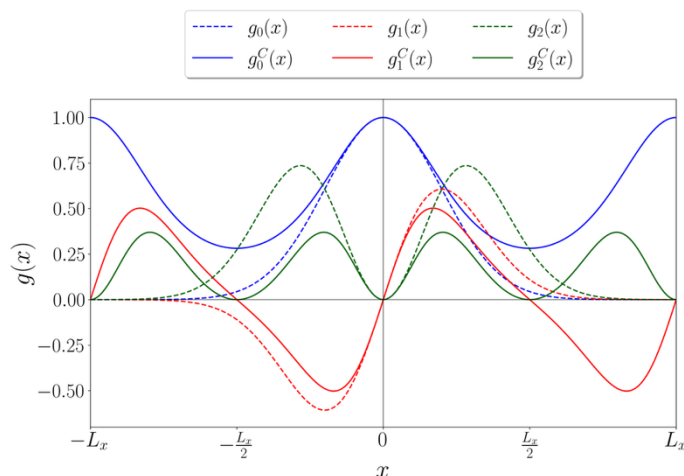
Fig : Periodic Clifford gaussians g_i^C(x) (solid lines) compared to regular non-periodic gaussians g_i(x) (dashed lines) in two neighboring supercells of length L_x for various values of i .
